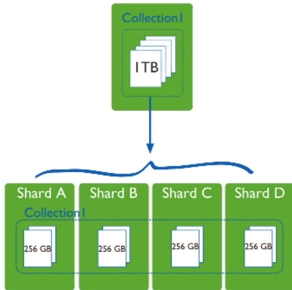
Figura 30. Sharding
